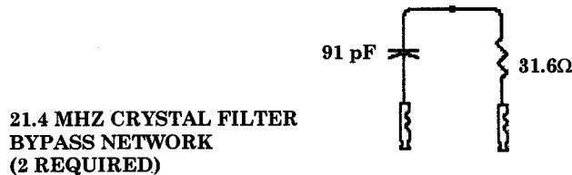
Figure 18. 21.4 MHz filter.
