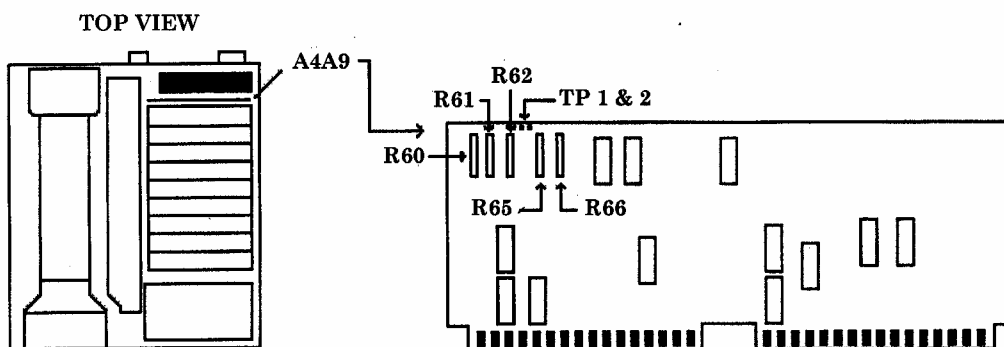
Figure 8. A4A9 board.
