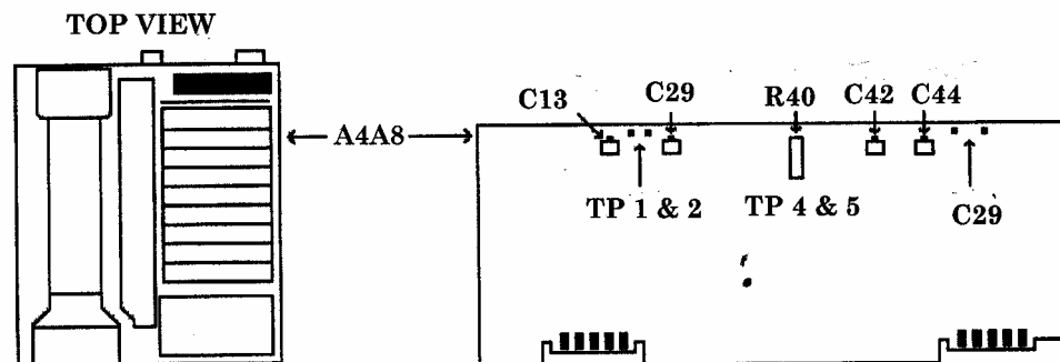
Figure 20. A4A8 board.
